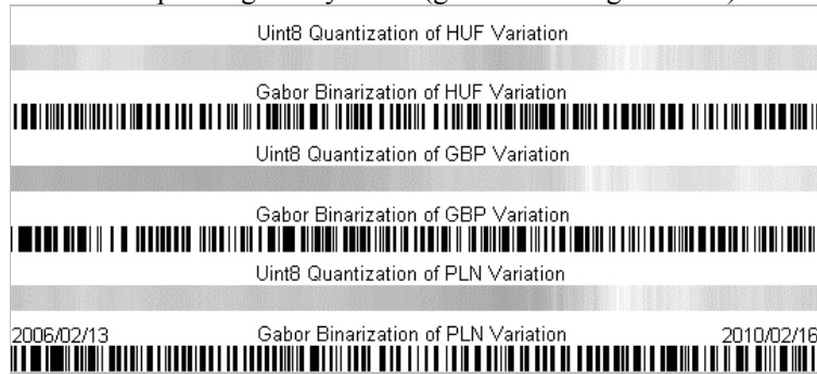
Figure 2. Uint8 quantization of three currency variation curves (HUF, GBP, PLN) and their corresponding binary codes (generated using GAPBE).
